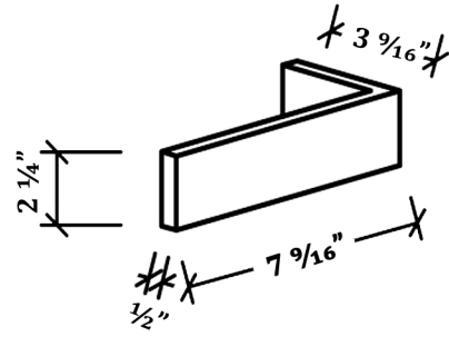
PUEBLO PLANT THIN BRICK CORNER
