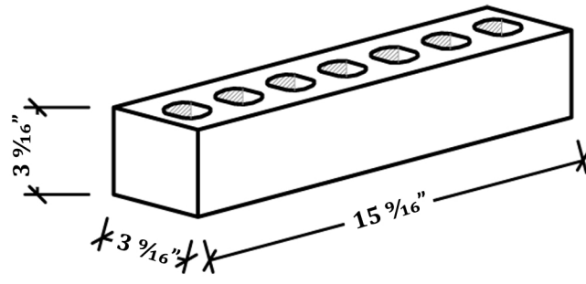
PUEBLO PLANT SUPER FOUR INCH (4x4x16)
