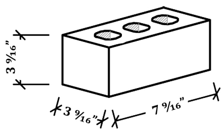
PUEBLO PLANT CLOSURE (4x4x8)
