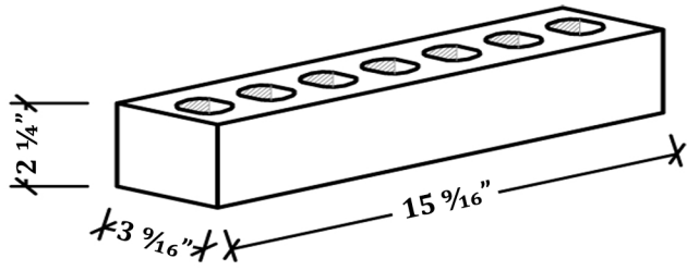
PUEBLO PLANT SUPER SIXTEEN INCH NORMAN
