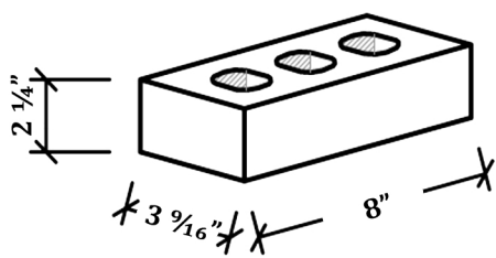
PUEBLO PLANT EIGHT INCH MODULAR
